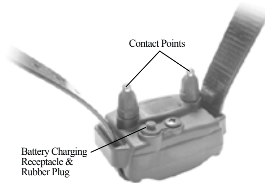
Receiver/Collar
