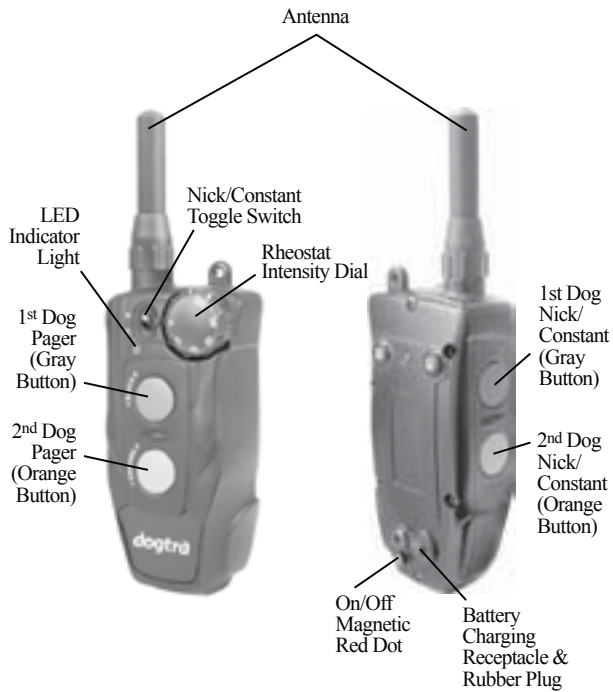
612C Transmitter
